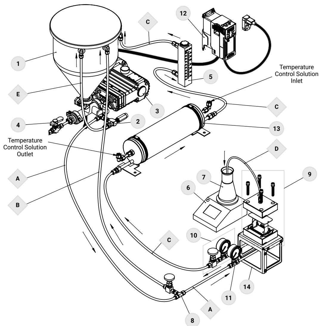
Figure 2: Cross Flow System Diagram for CF042A Cell
