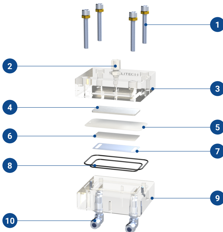
Figure 1: CF042A Cross Flow Cell Body Assembly
