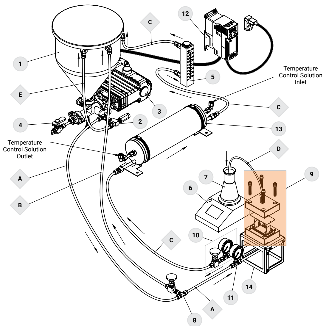
Figure 2: Cross Flow System Diagram for CF042SS Cell
