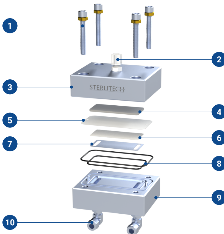
Figure 1: CF042SS Crossflow Cell Body Assembly
