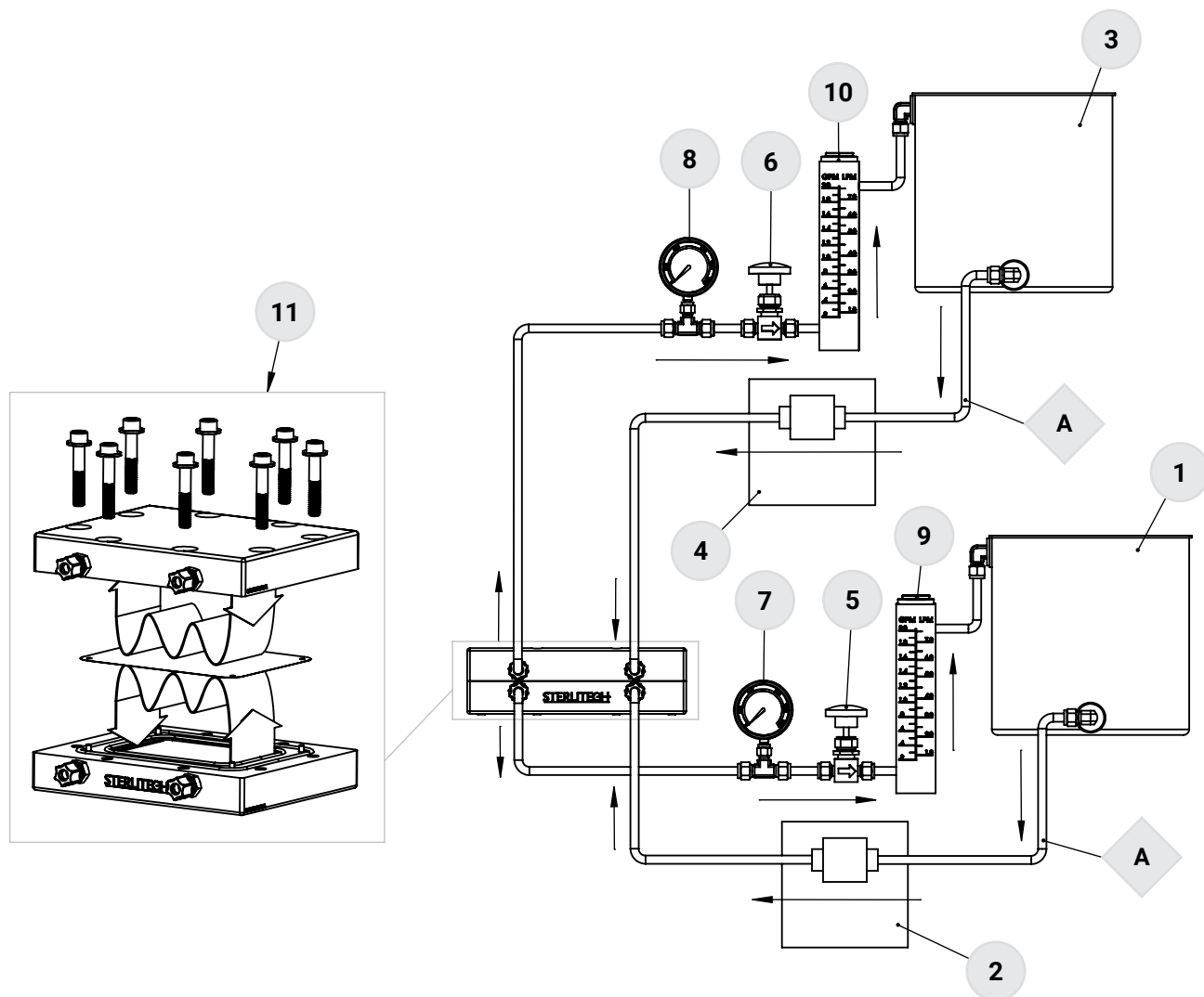
Figure 2: Forward Osmosis System Flow Diagram For Sepa Cell
