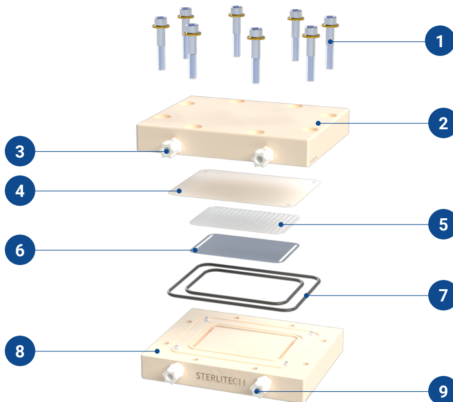
Figure 1: PEEK Sepa FO Cell Body Assembly
