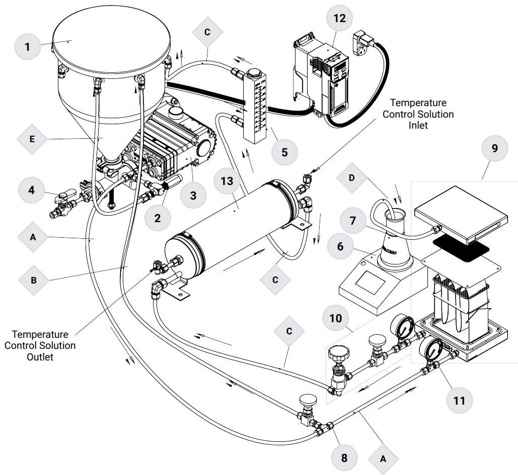
Figure 2: Cross Flow System Diagram for Acrylic Sepa CF Cell
