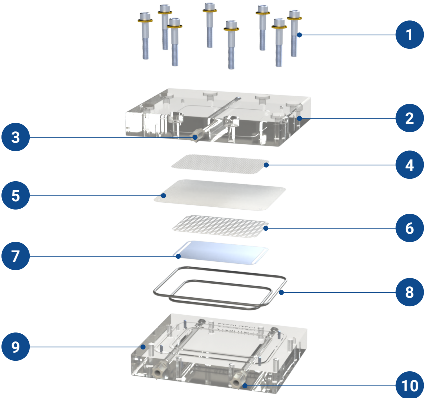
Figure 1: Acrylic Sepa CF Cell Body Assembly
